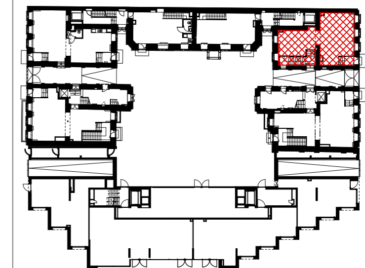
SCHEMAT PARTERU
