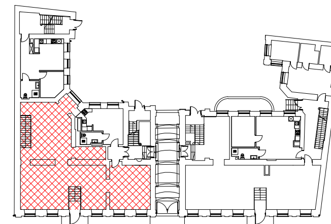
SCHEMAT PARTERU
